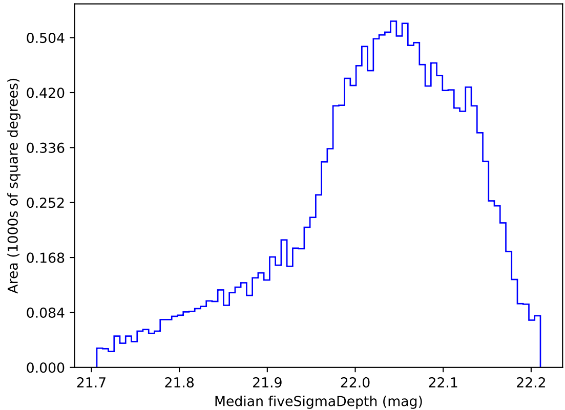
too_elab_2yr_r128_d3_griz_v3.4_10yrs WFD y band: Median fiveSigmaDepth
