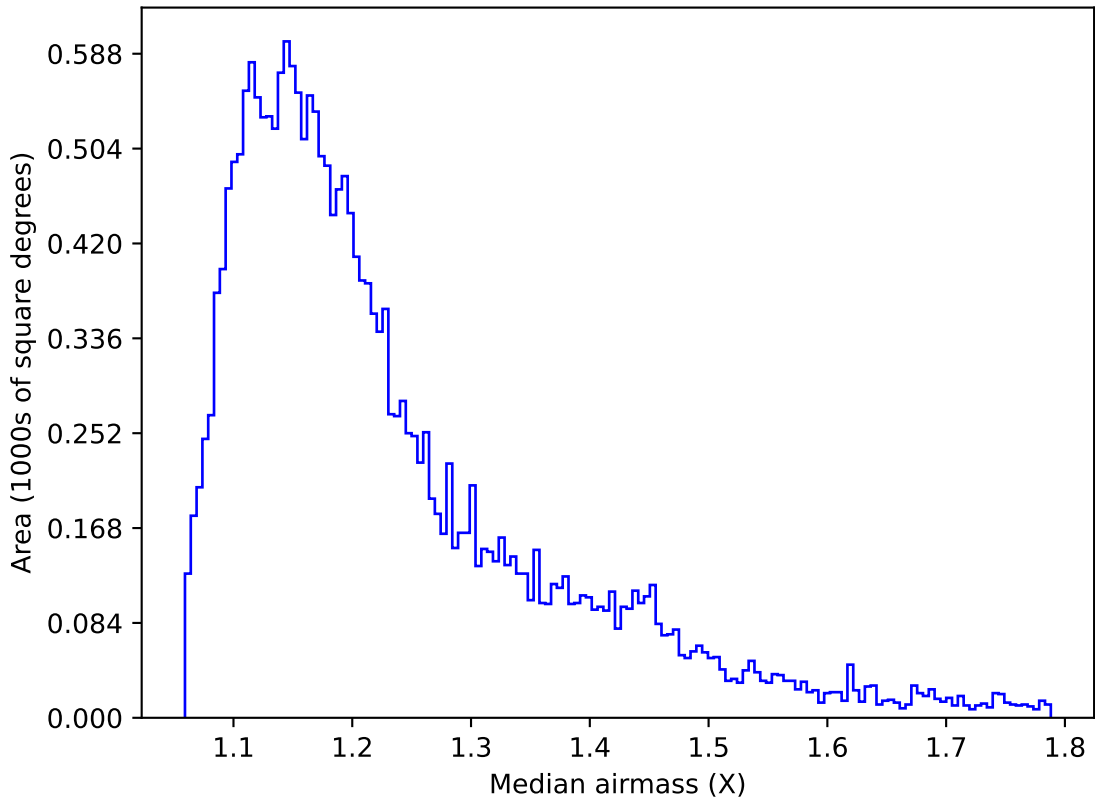
too_elab_2yr_r128_d3_griz_v3.4_10yrs Yr 1 u band: Median airmass
