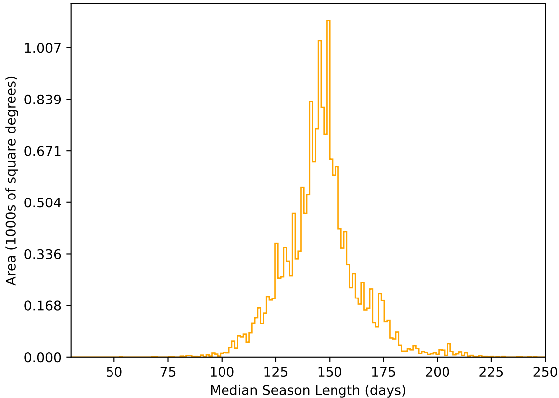
too_elab_2yr_r128_d3_griz_v3.4_10yrs WFD r band: Median Season Length
