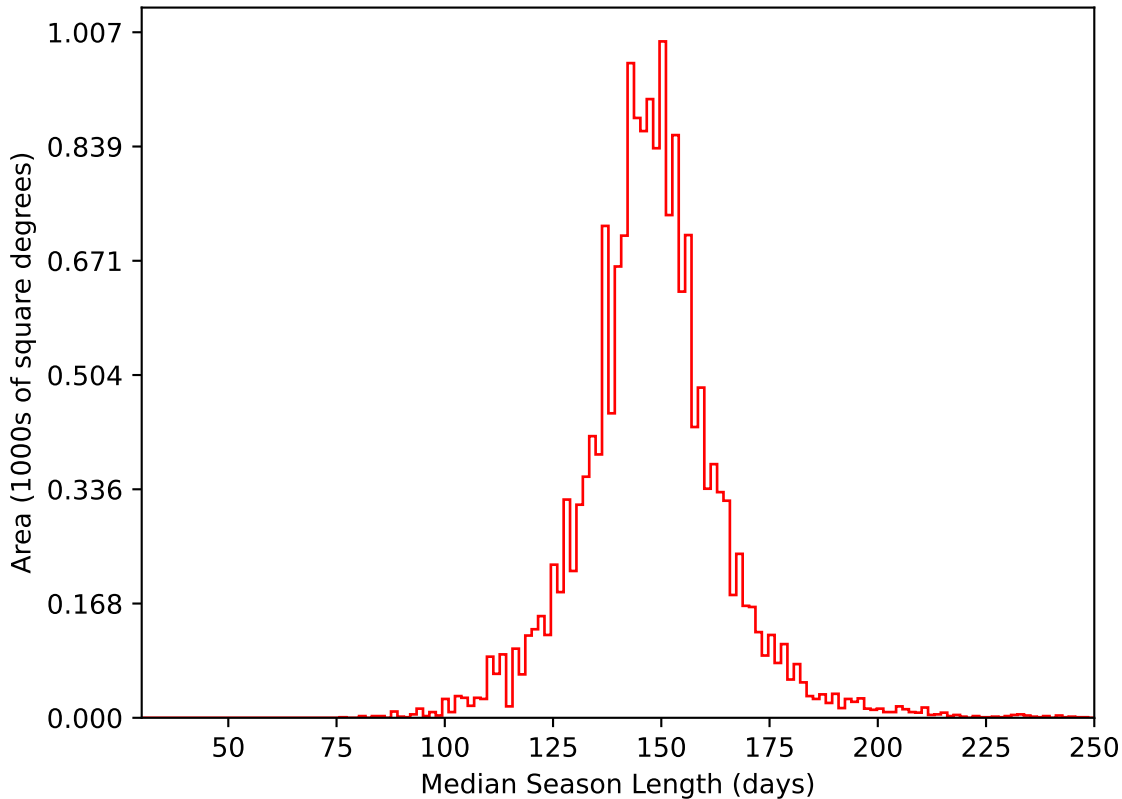
too_elab_2yr_r128_d3_griz_v3.4_10yrs WFD i band: Median Season Length
