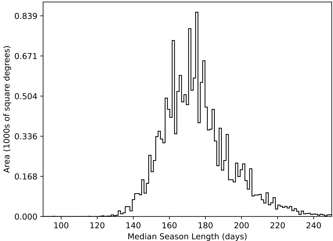
too_elab_2yr_r128_d3_griz_v3.4_10yrs WFD all bands: Median Season Length
