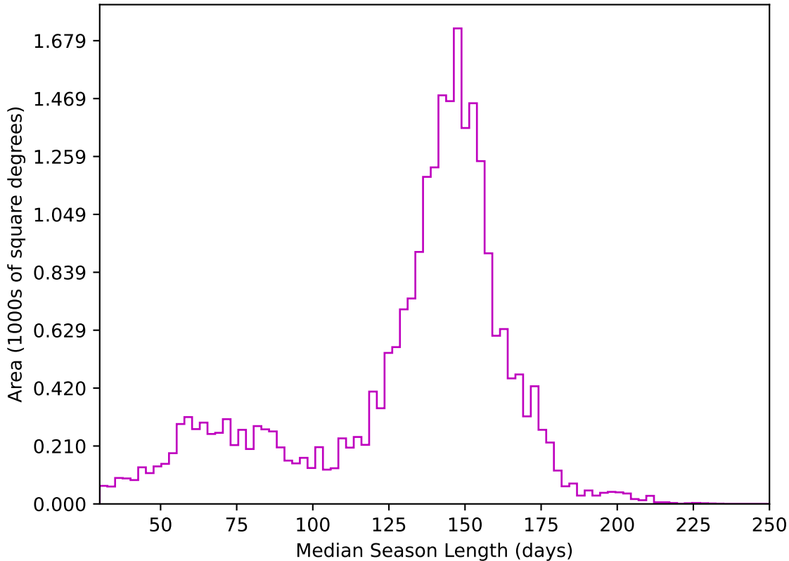
too_elab_2yr_r128_d3_griz_v3.4_10yrs All sky z band: Median Season Length
