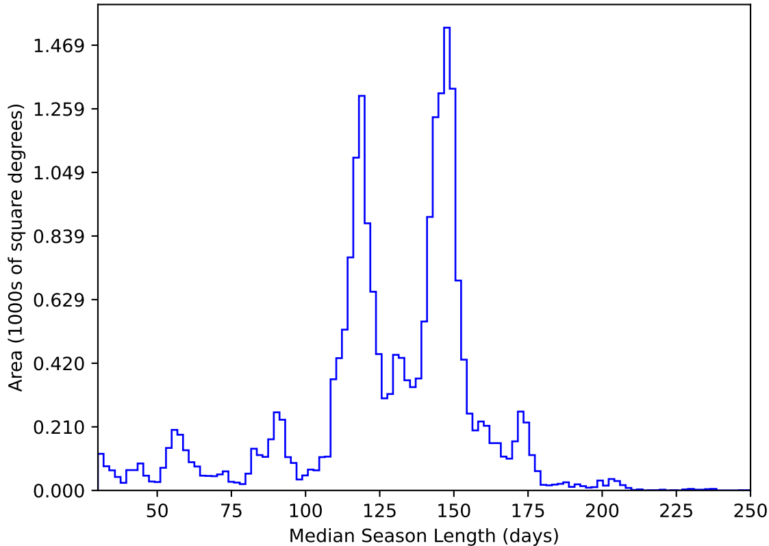
too_elab_2yr_r128_d3_griz_v3.4_10yrs All sky y band: Median Season Length
