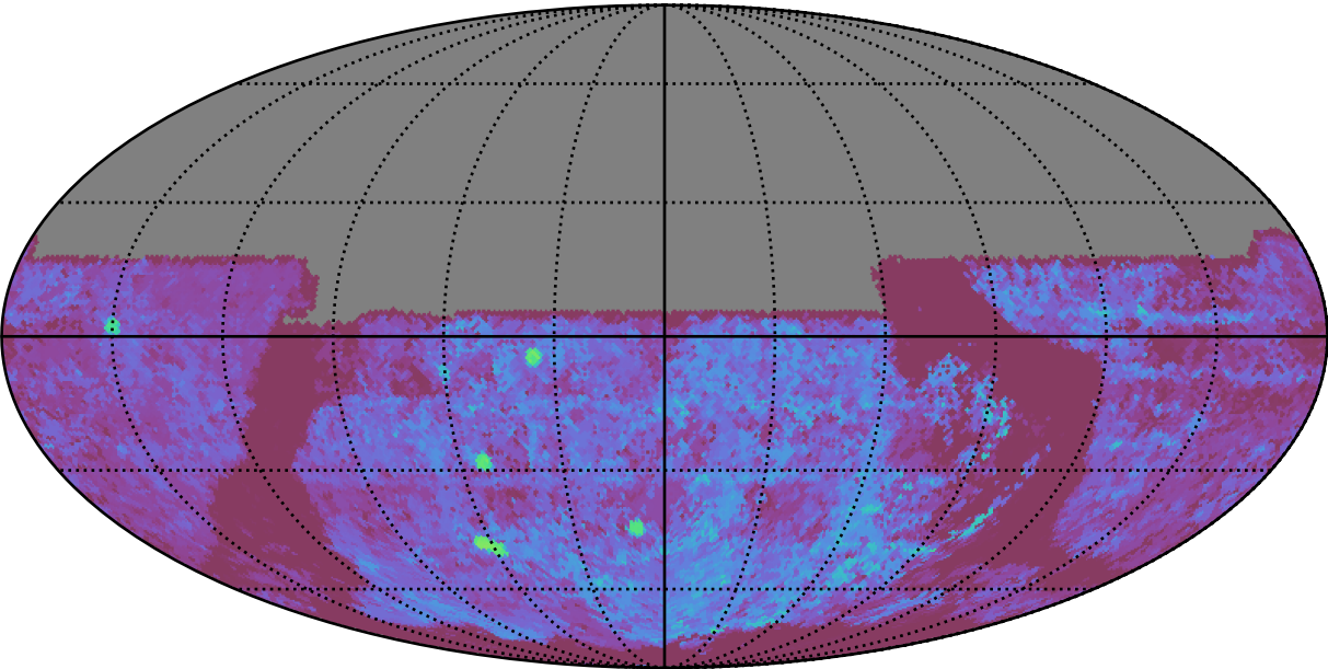
too_elab_2yr_r128_d3_griz_v3.4_10yrs All sky u band: Median Season Length
