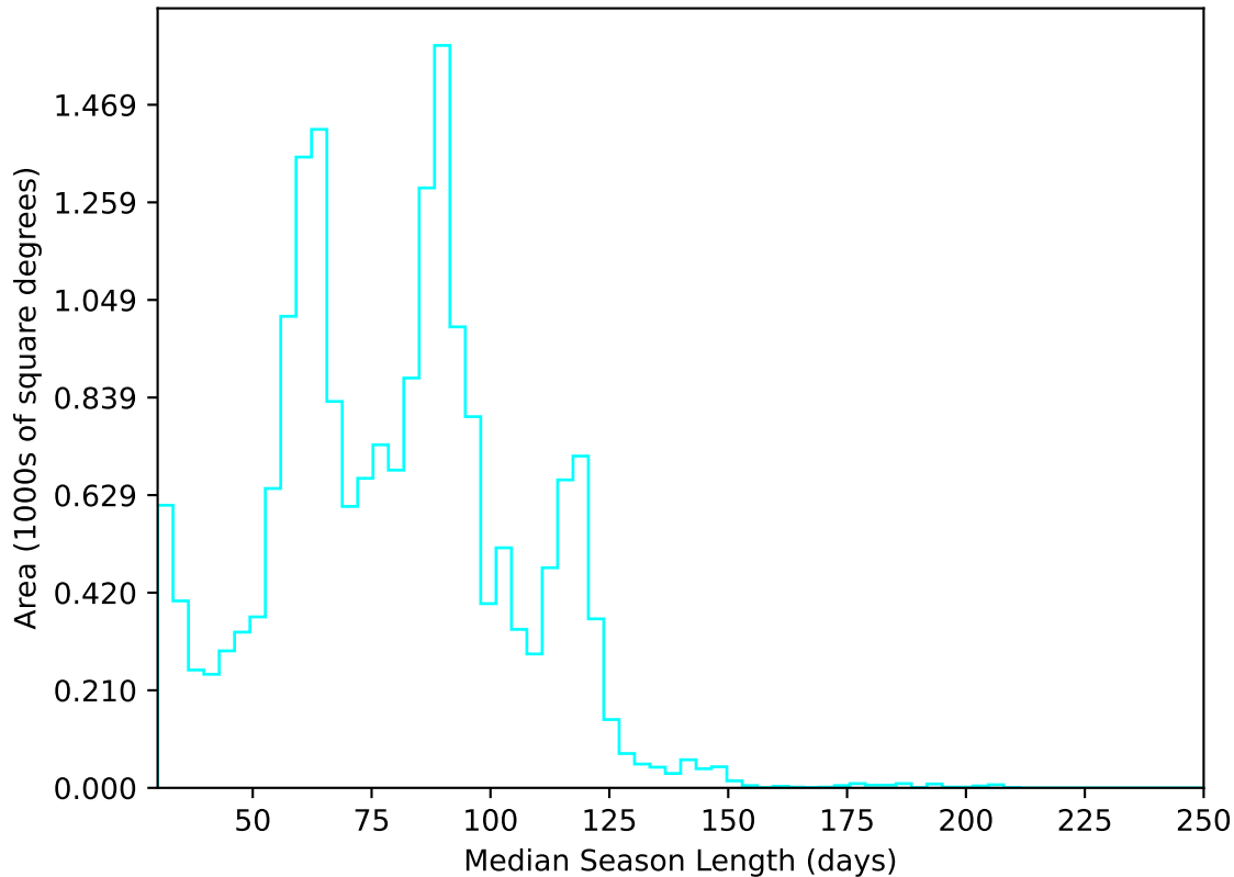
too_elab_2yr_r128_d3_griz_v3.4_10yrs All sky u band: Median Season Length
