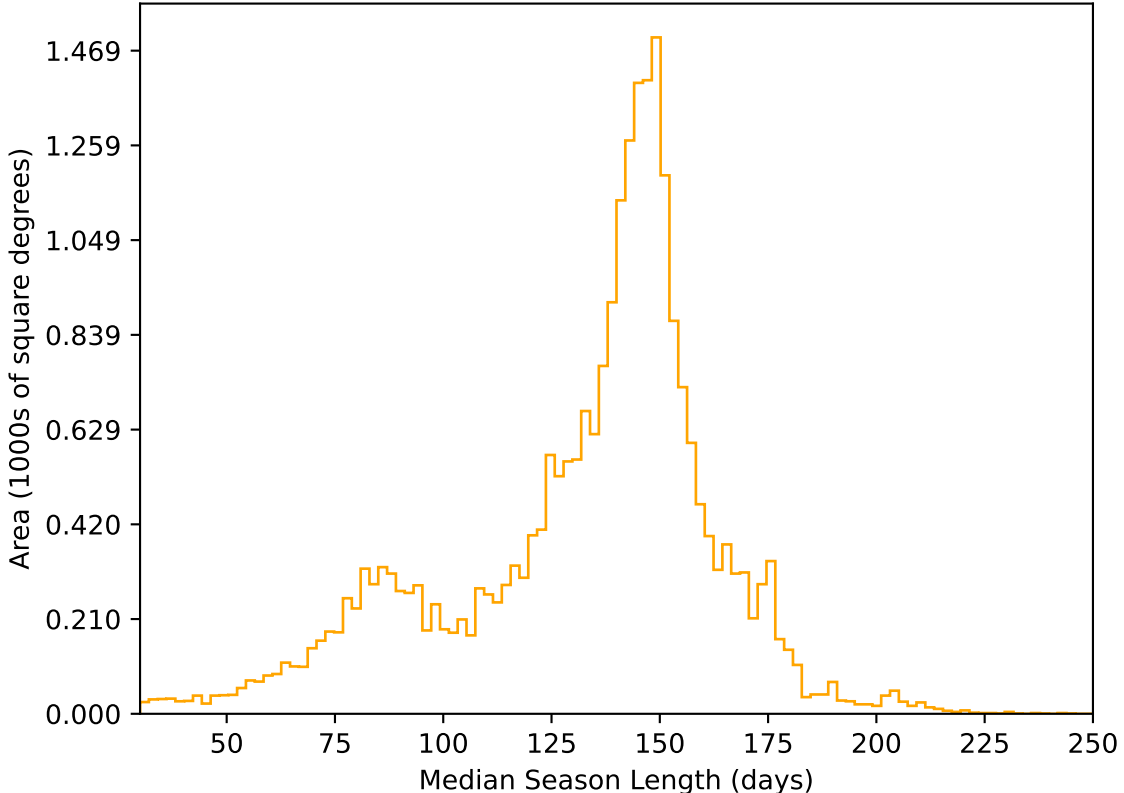
too_elab_2yr_r128_d3_griz_v3.4_10yrs All sky r band: Median Season Length
