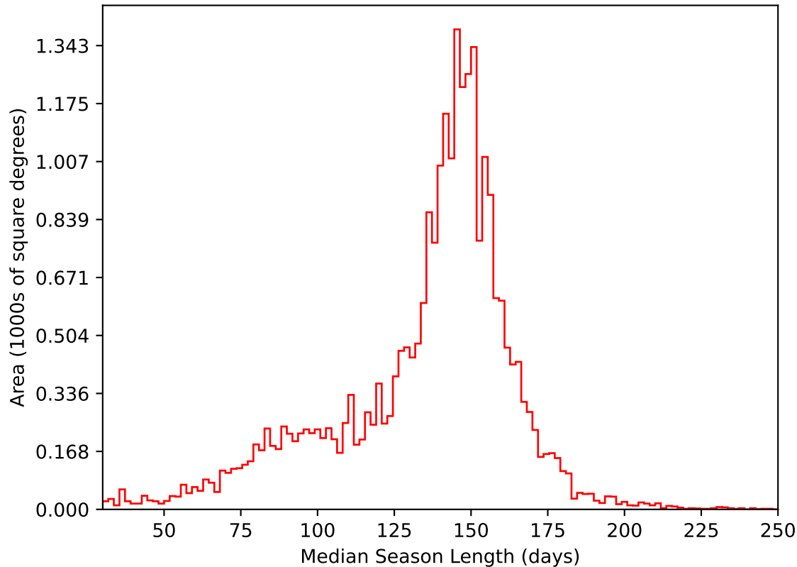
too_elab_2yr_r128_d3_griz_v3.4_10yrs All sky i band: Median Season Length
