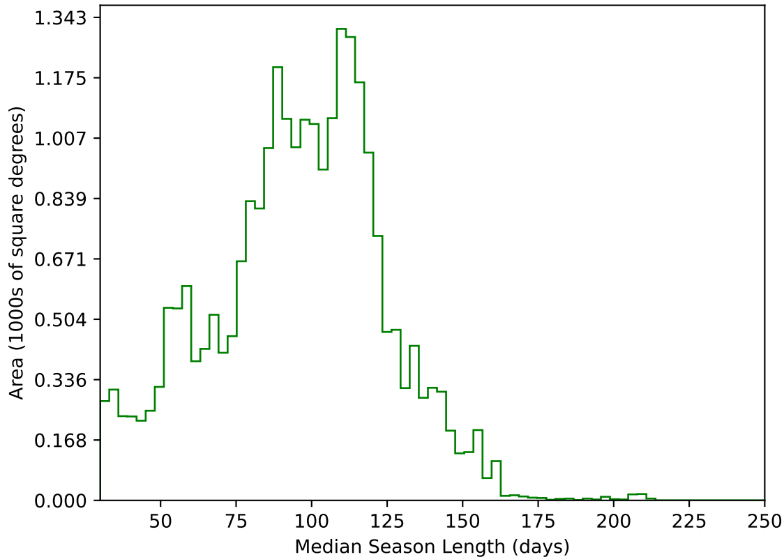
too_elab_2yr_r128_d3_griz_v3.4_10yrs All sky g band: Median Season Length
