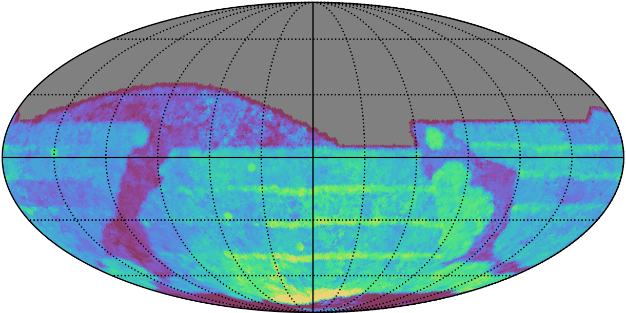
too_elab_2yr_r128_d3_griz_v3.4_10yrs All sky all bands: Median Season Length
