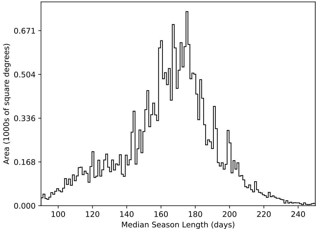
too_elab_2yr_r128_d3_griz_v3.4_10yrs All sky all bands: Median Season Length
