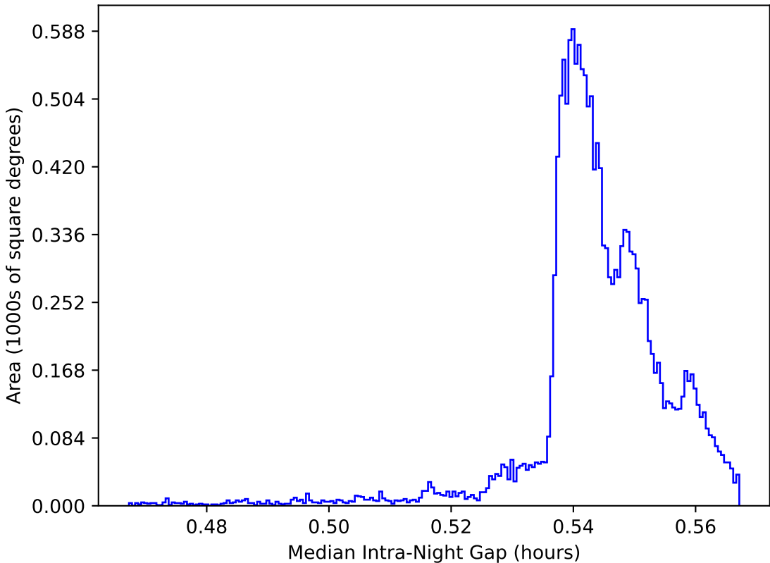
too_elab_2yr_r128_d3_griz_v3.4_10yrs WFD: Median Intra-Night Gap
