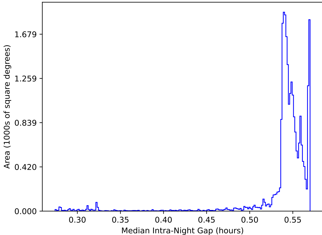
too_elab_2yr_r128_d3_griz_v3.4_10yrs All sky: Median Intra-Night Gap
