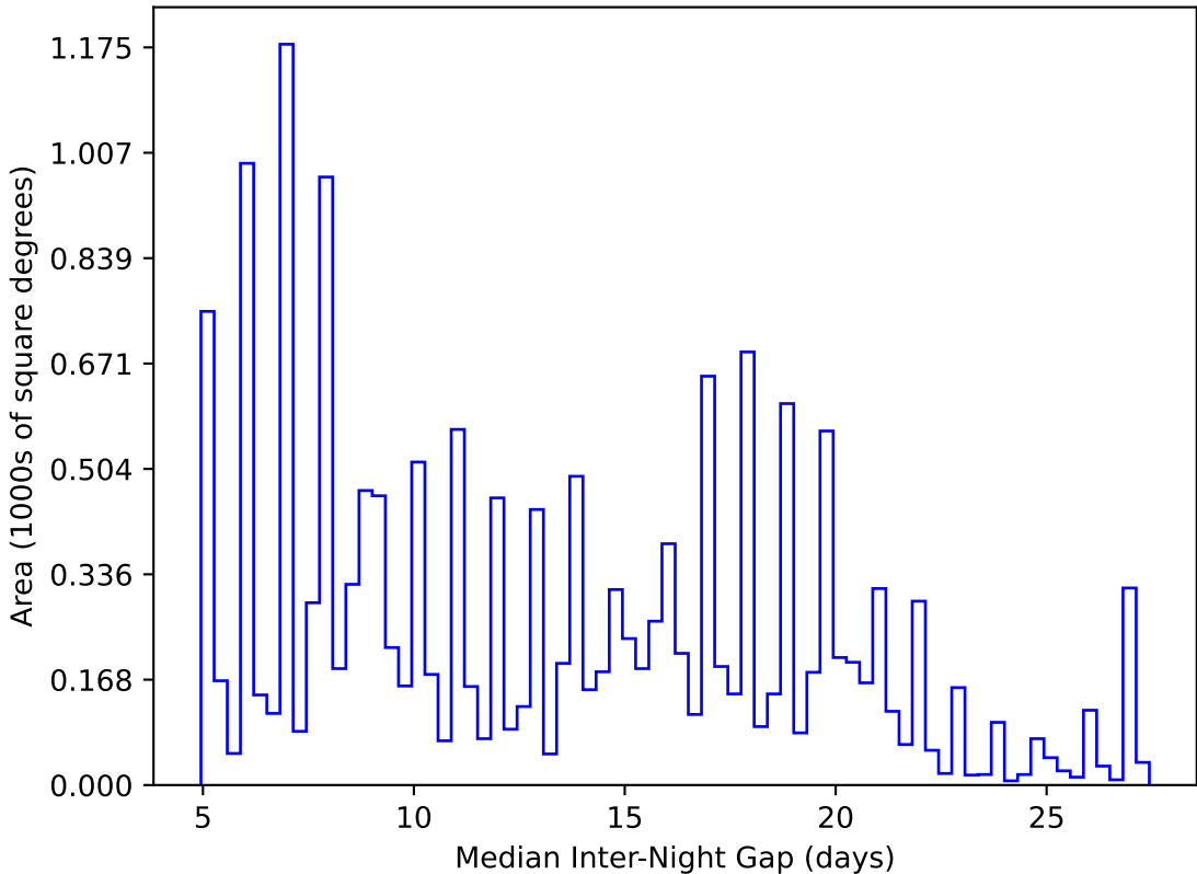
too_elab_2yr_r128_d3_griz_v3.4_10yrs WFD y band: Median Inter-Night Gap
