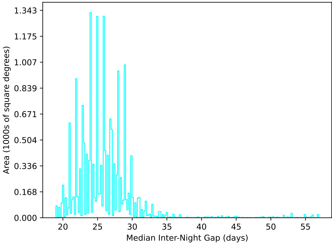
too_elab_2yr_r128_d3_griz_v3.4_10yrs WFD u band: Median Inter-Night Gap
