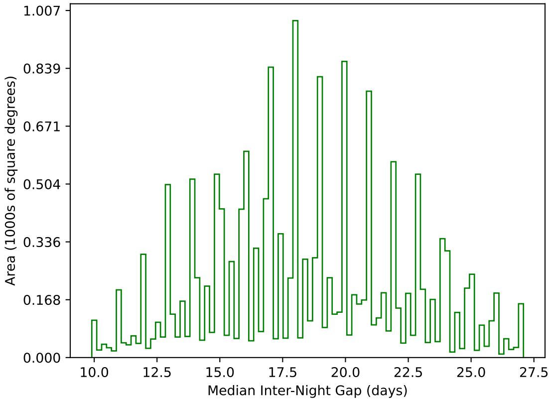
too_elab_2yr_r128_d3_griz_v3.4_10yrs WFD g band: Median Inter-Night Gap
