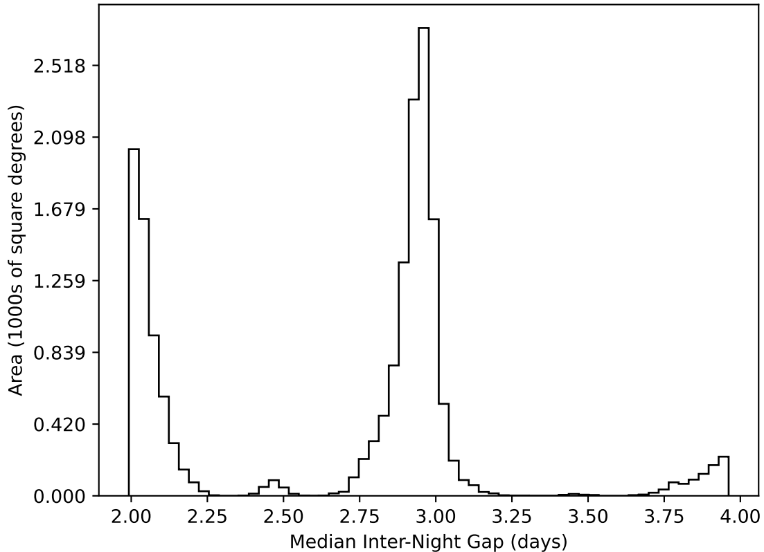
too_elab_2yr_r128_d3_griz_v3.4_10yrs WFD all bands: Median Inter-Night Gap
