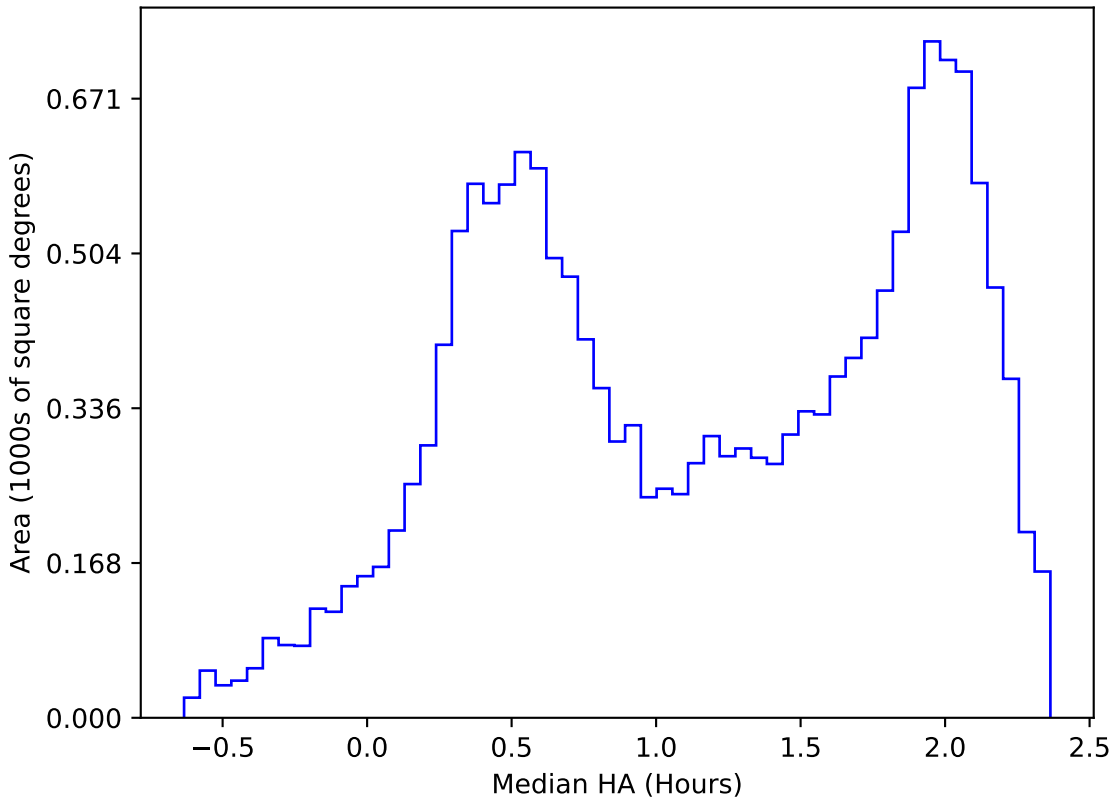
too_elab_2yr_r128_d3_griz_v3.4_10yrs WFD z band: Median HA
