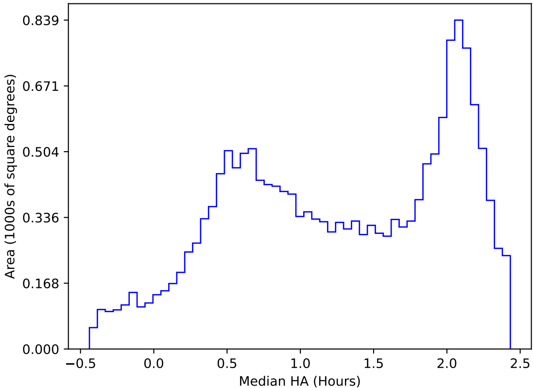
too_elab_2yr_r128_d3_griz_v3.4_10yrs WFD y band: Median HA
