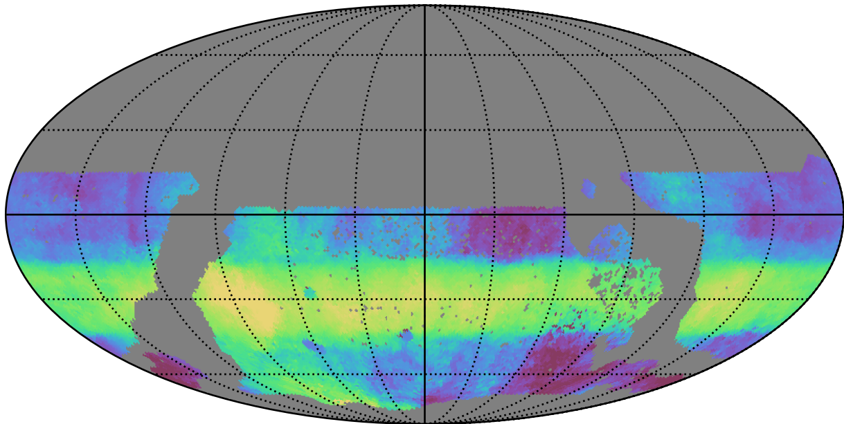
too_elab_2yr_r128_d3_griz_v3.4_10yrs WFD r band: Median HA
