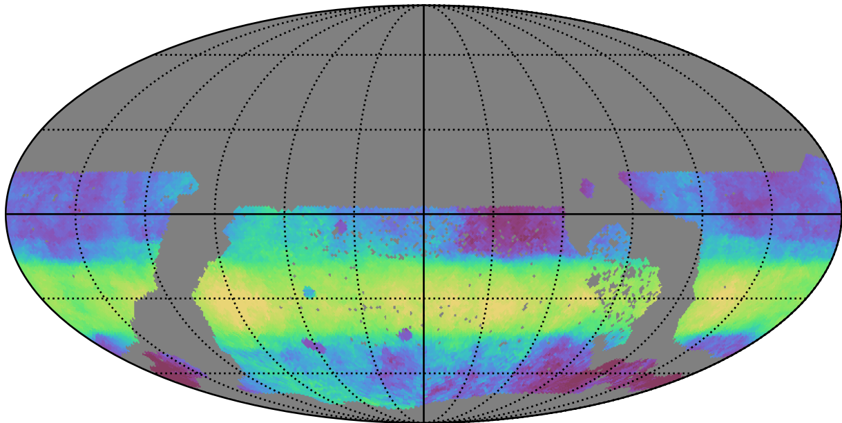
too_elab_2yr_r128_d3_griz_v3.4_10yrs WFD i band: Median HA
