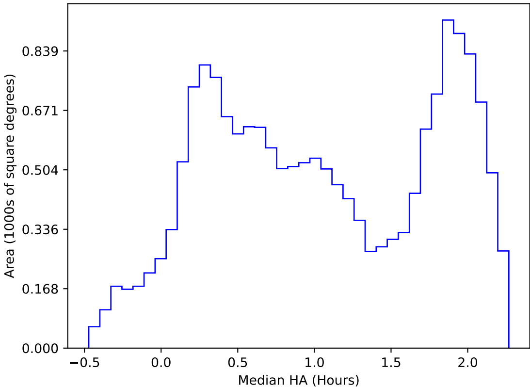
too_elab_2yr_r128_d3_griz_v3.4_10yrs WFD i band: Median HA
