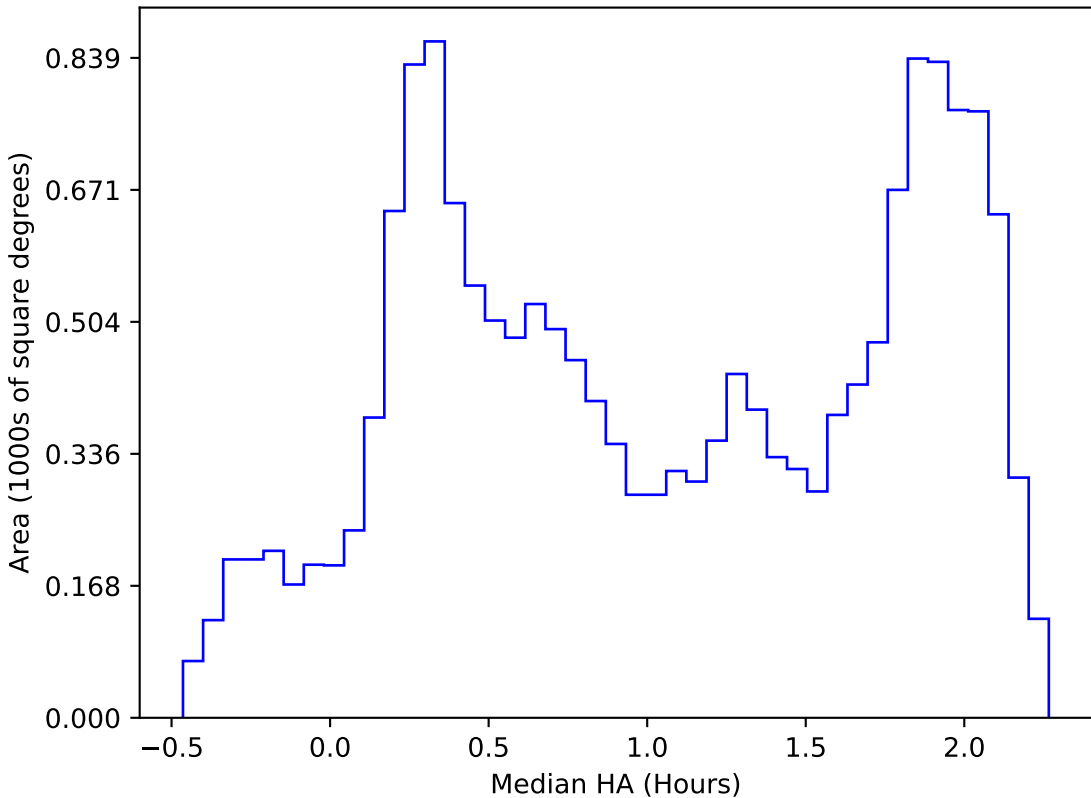
too_elab_2yr_r128_d3_griz_v3.4_10yrs WFD all bands: Median HA
