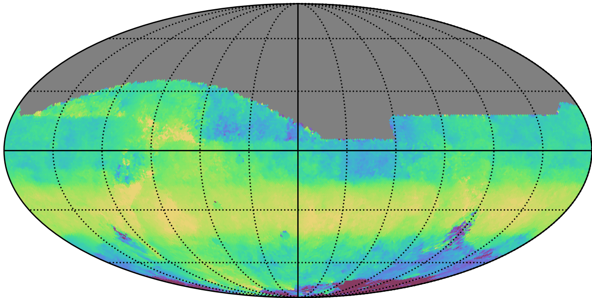
too_elab_2yr_r128_d3_griz_v3.4_10yrs All sky z band: Median HA
