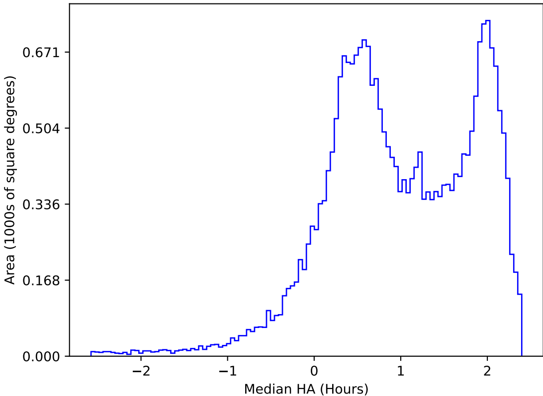
too_elab_2yr_r128_d3_griz_v3.4_10yrs All sky z band: Median HA
