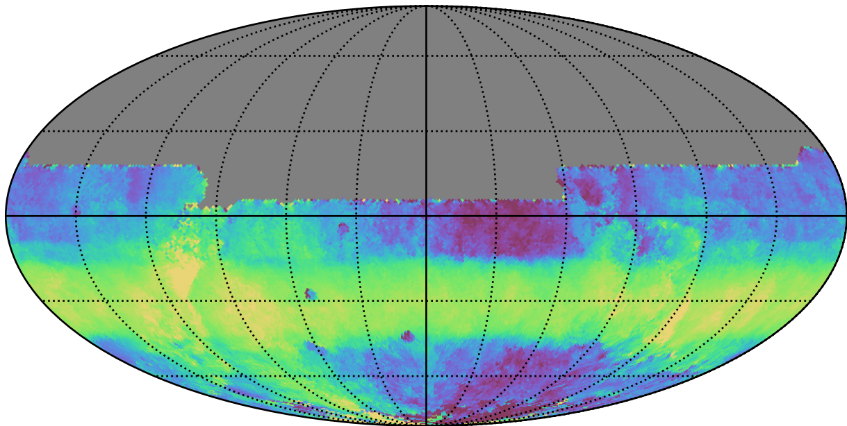
too_elab_2yr_r128_d3_griz_v3.4_10yrs All sky y band: Median HA
