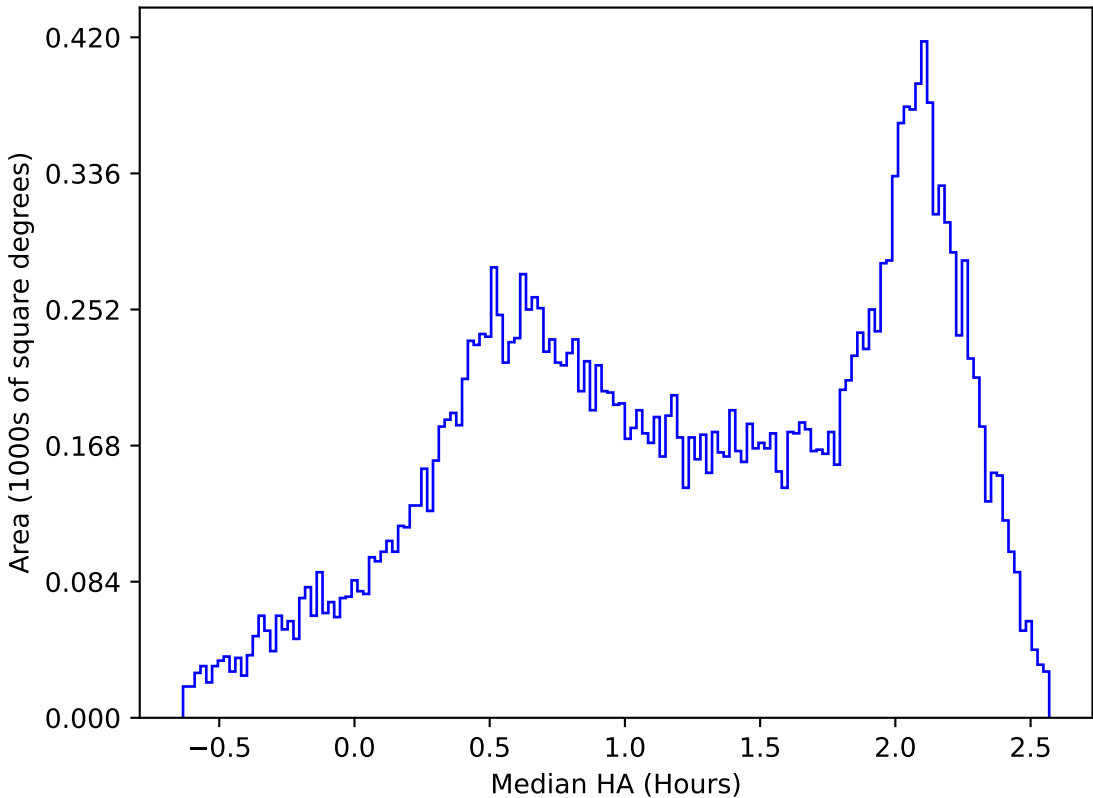
too_elab_2yr_r128_d3_griz_v3.4_10yrs All sky y band: Median HA
