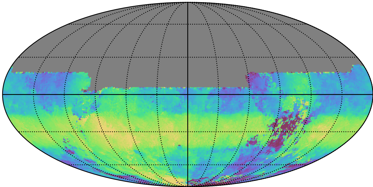
too_elab_2yr_r128_d3_griz_v3.4_10yrs All sky u band: Median HA
