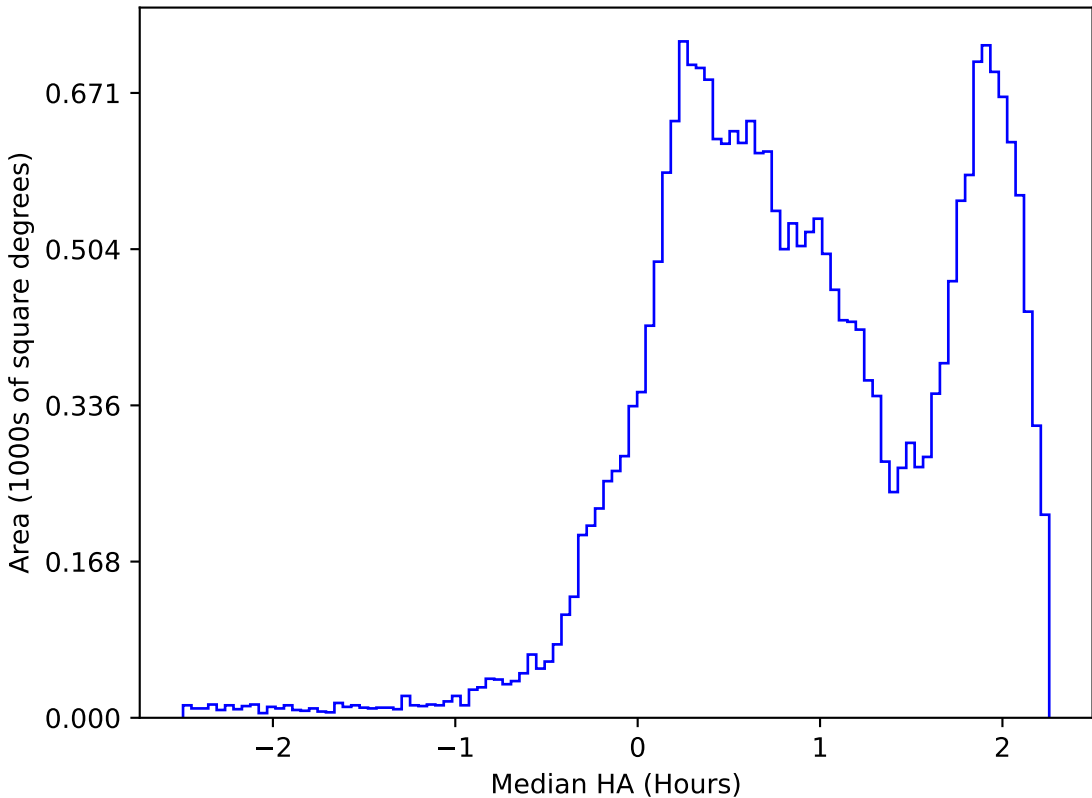
too_elab_2yr_r128_d3_griz_v3.4_10yrs All sky i band: Median HA
