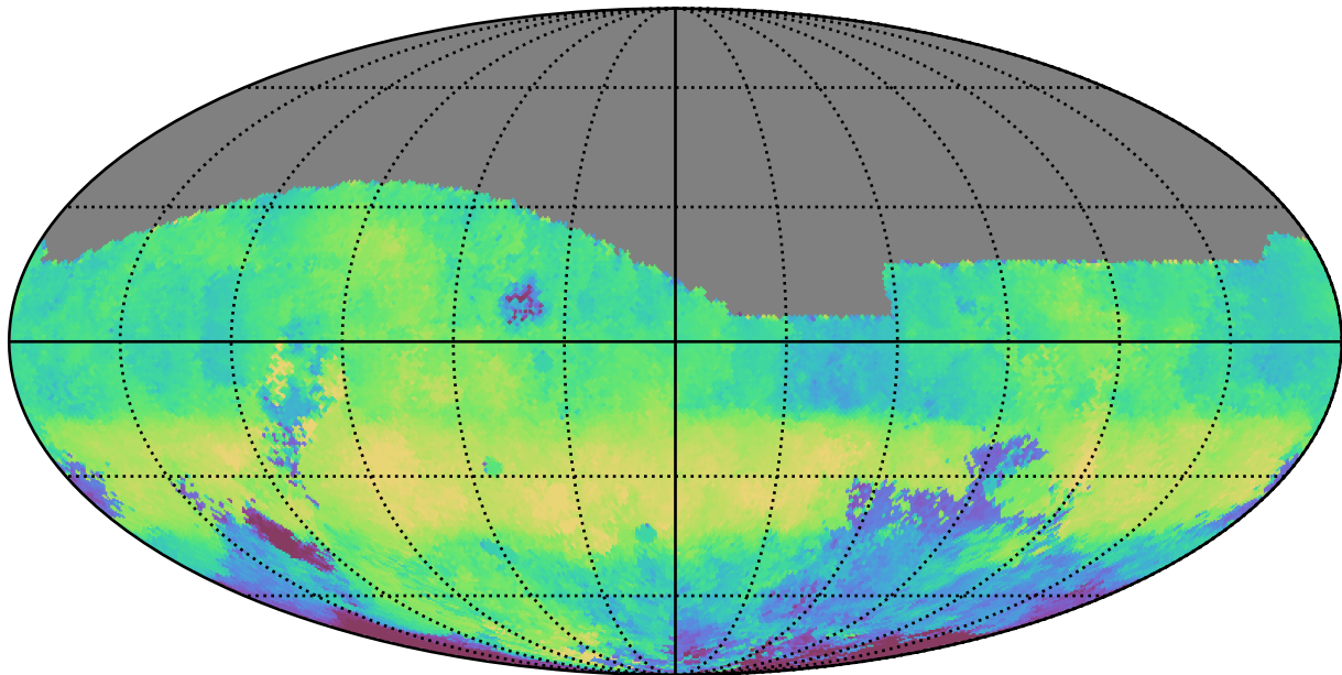
too_elab_2yr_r128_d3_griz_v3.4_10yrs All sky g band: Median HA
