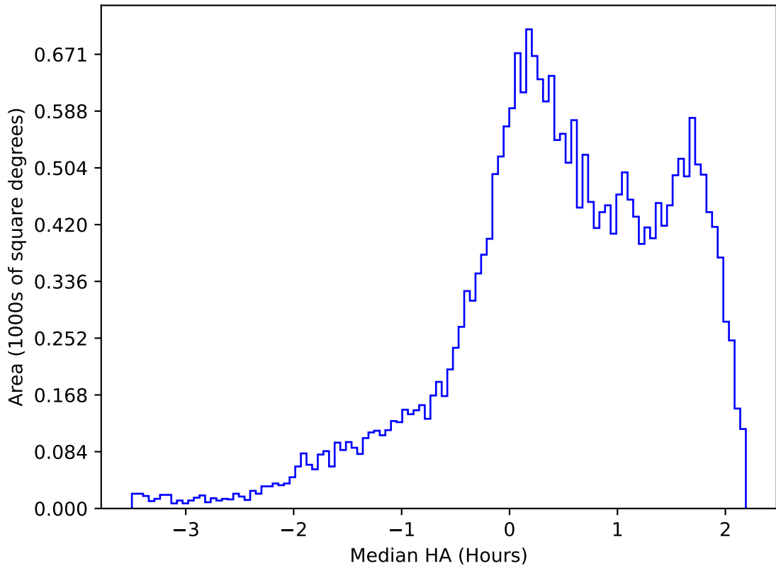
too_elab_2yr_r128_d3_griz_v3.4_10yrs All sky g band: Median HA
