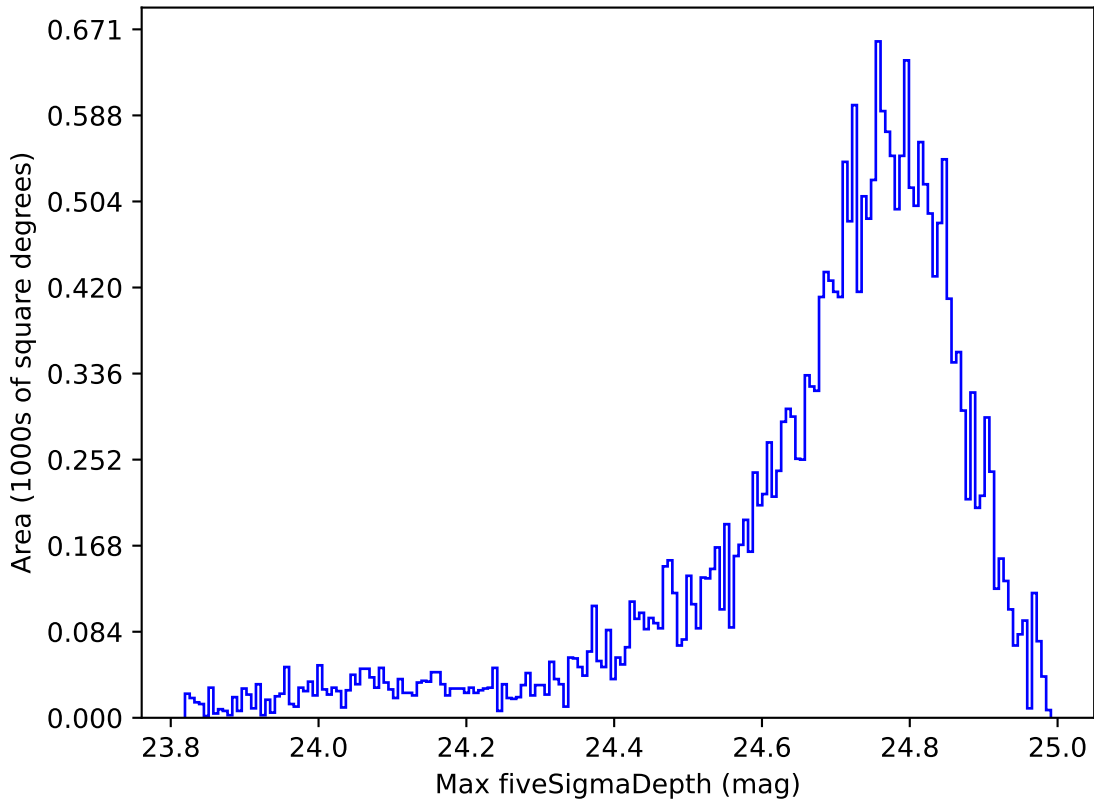
too_elab_2yr_r128_d3_griz_v3.4_10yrs All sky r band: Max fiveSigmaDepth
