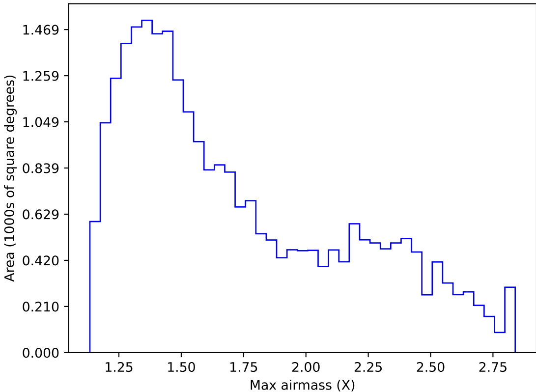
too_elab_2yr_r128_d3_griz_v3.4_10yrs Yr 1 z band: Max airmass
