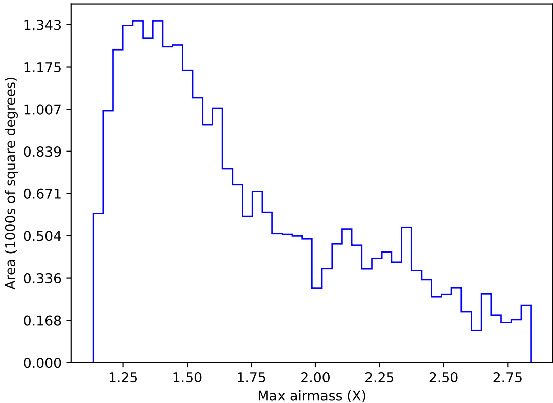
too_elab_2yr_r128_d3_griz_v3.4_10yrs Yr 1 i band: Max airmass
