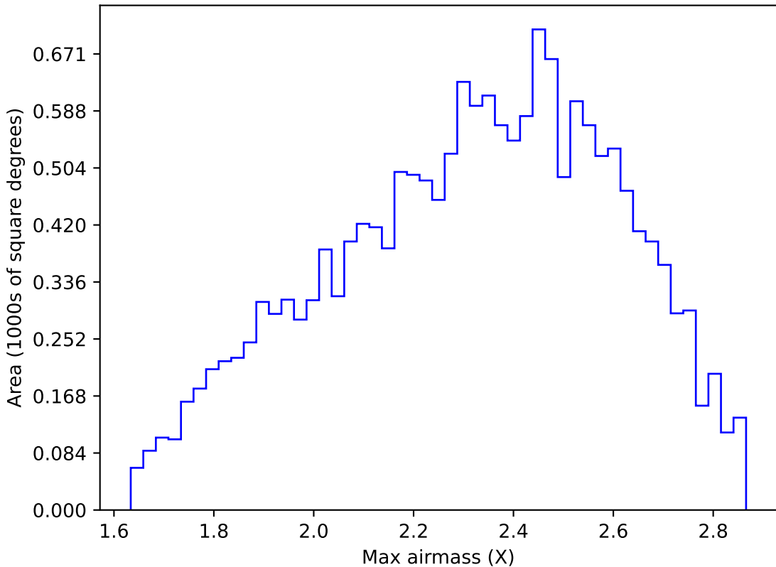
too_elab_2yr_r128_d3_griz_v3.4_10yrs WFD y band: Max airmass
