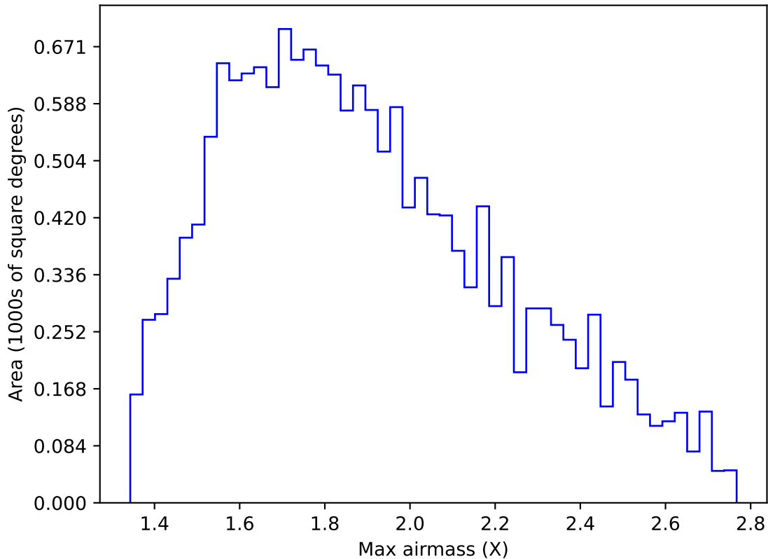
too_elab_2yr_r128_d3_griz_v3.4_10yrs WFD u band: Max airmass
