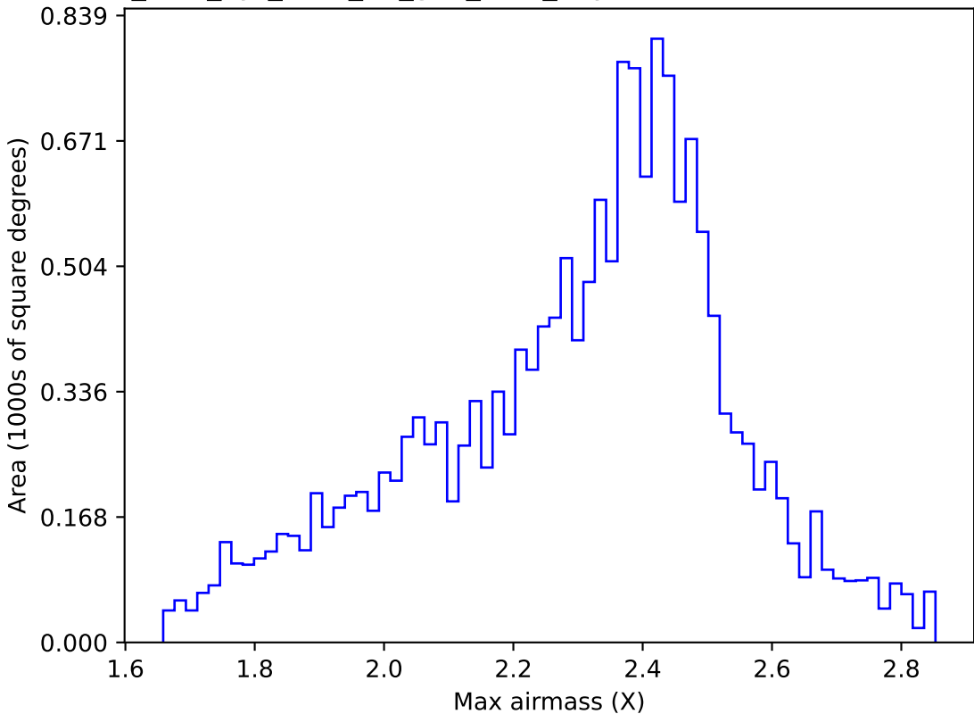
too_elab_2yr_r128_d3_griz_v3.4_10yrs WFD r band: Max airmass
