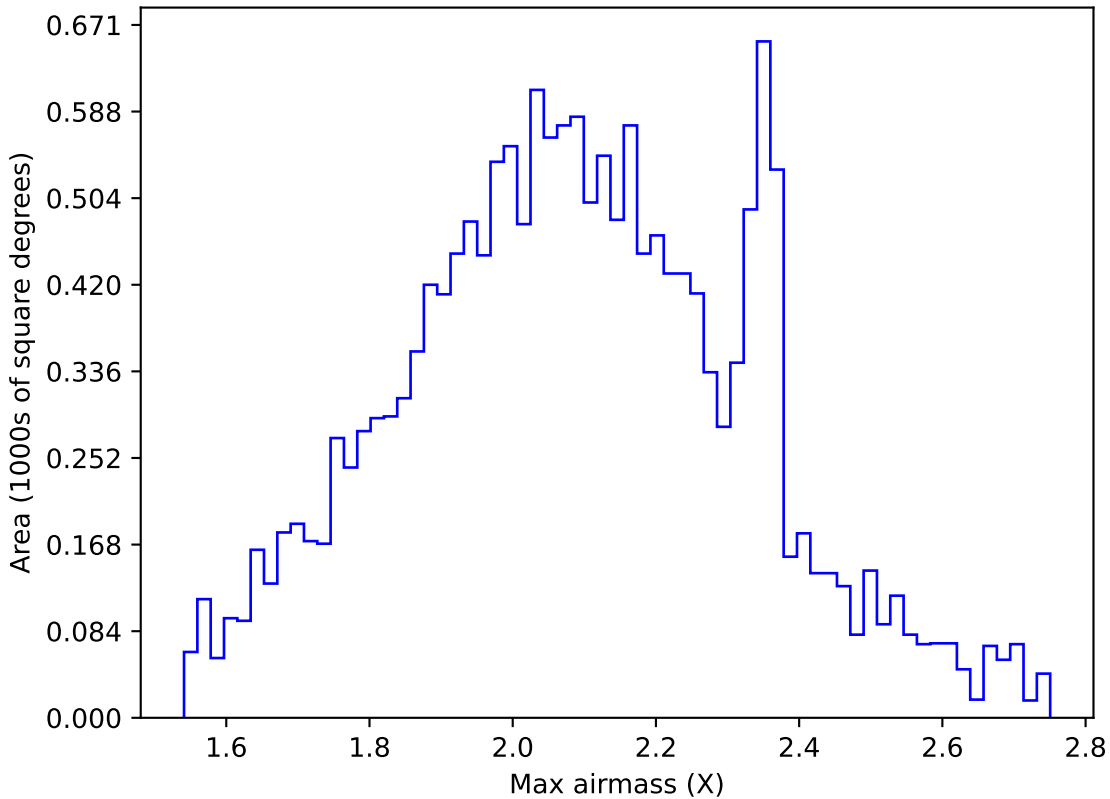
too_elab_2yr_r128_d3_griz_v3.4_10yrs WFD g band: Max airmass
