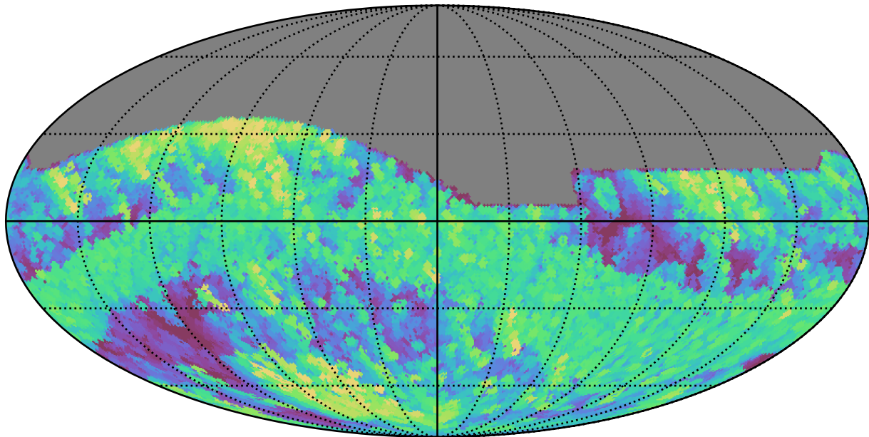
too_elab_2yr_r128_d3_griz_v3.4_10yrs All sky r band: Max airmass
