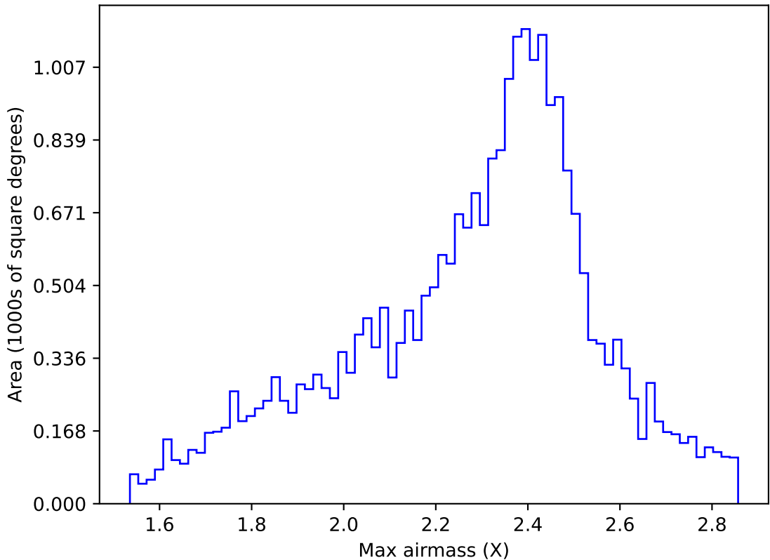
too_elab_2yr_r128_d3_griz_v3.4_10yrs All sky r band: Max airmass
