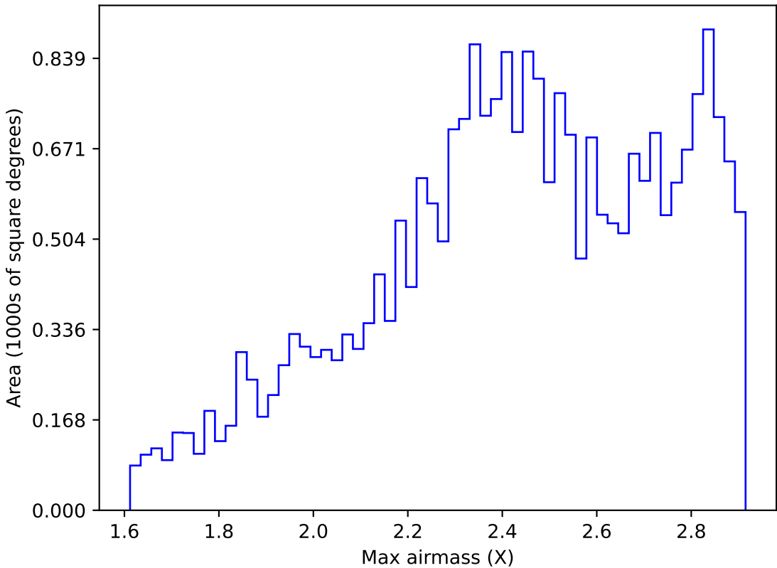
too_elab_2yr_r128_d3_griz_v3.4_10yrs All sky i band: Max airmass
