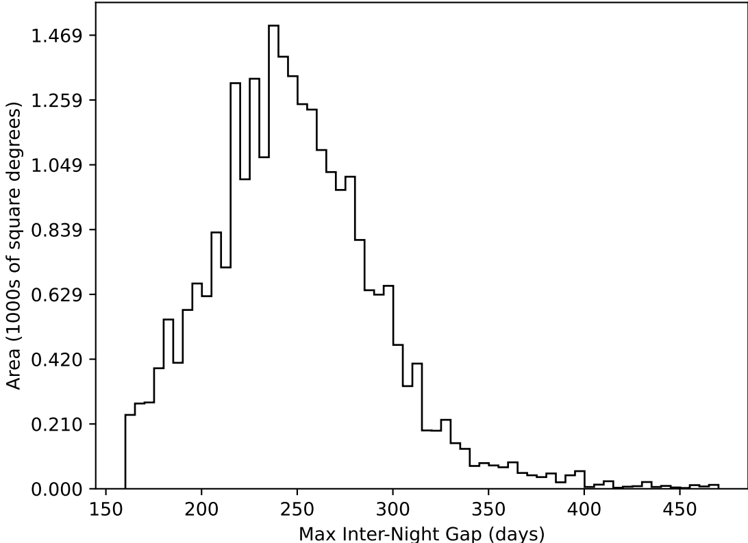
too_elab_2yr_r128_d3_griz_v3.4_10yrs All sky all bands: Max Inter-Night Gap
