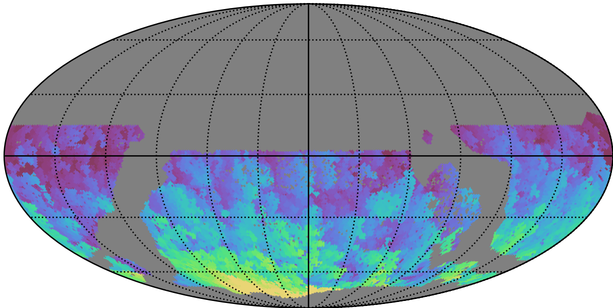
too_elab_2yr_r128_d3_griz_v3.4_10yrs WFD g band: Max HA
