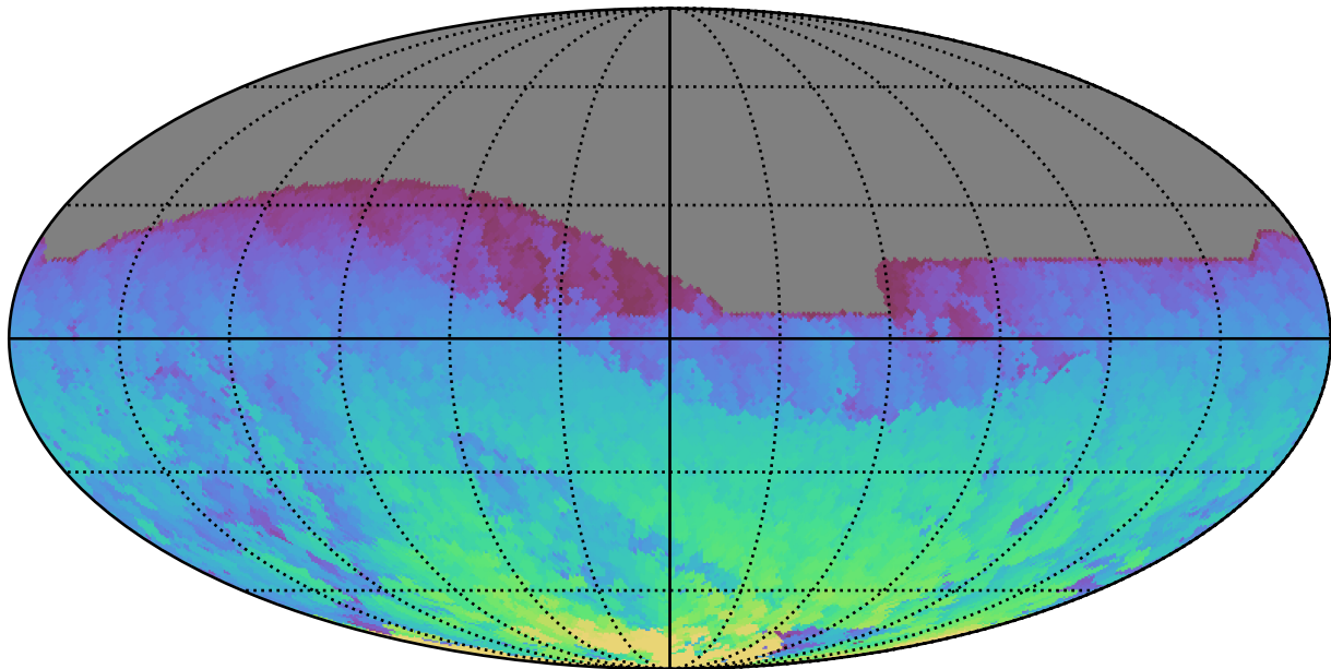
too_elab_2yr_r128_d3_griz_v3.4_10yrs All sky z band: Max HA
