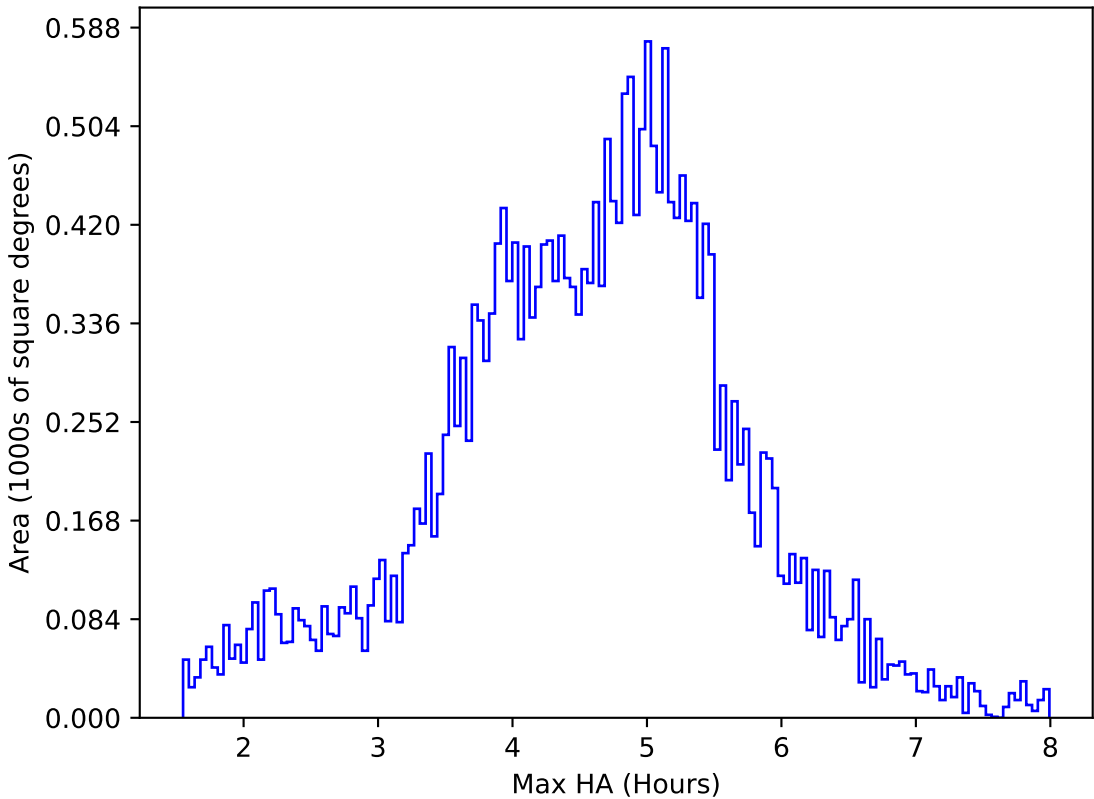
too_elab_2yr_r128_d3_griz_v3.4_10yrs All sky z band: Max HA
