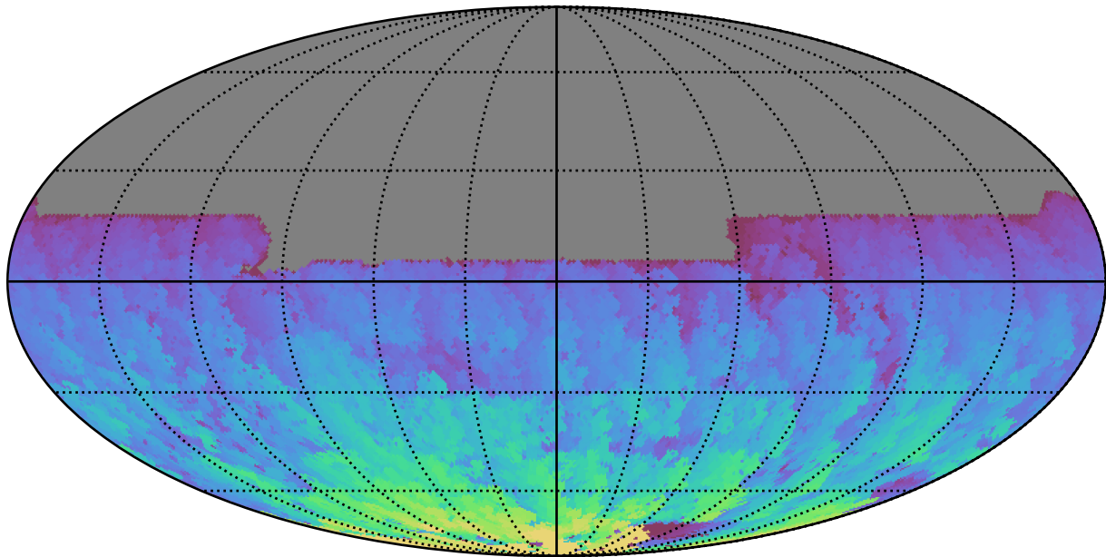
too_elab_2yr_r128_d3_griz_v3.4_10yrs All sky y band: Max HA
