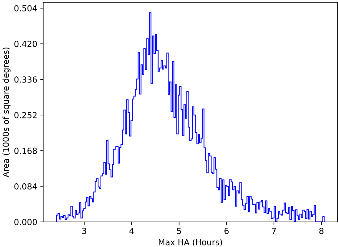
too_elab_2yr_r128_d3_griz_v3.4_10yrs All sky y band: Max HA
